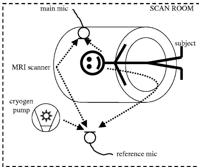
FIG. 3. Noise sources and microphone arrangement.
