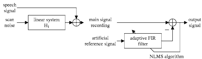
FIG. 5. Adaptive FIR filter using NLMS algorithm for model-based cancellation of interference from MRI scanner noise.
